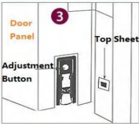
Insert the sealing strip and fix the top piece
