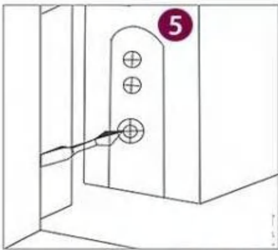
Rotation adjustment to close the door Seal to floor position
